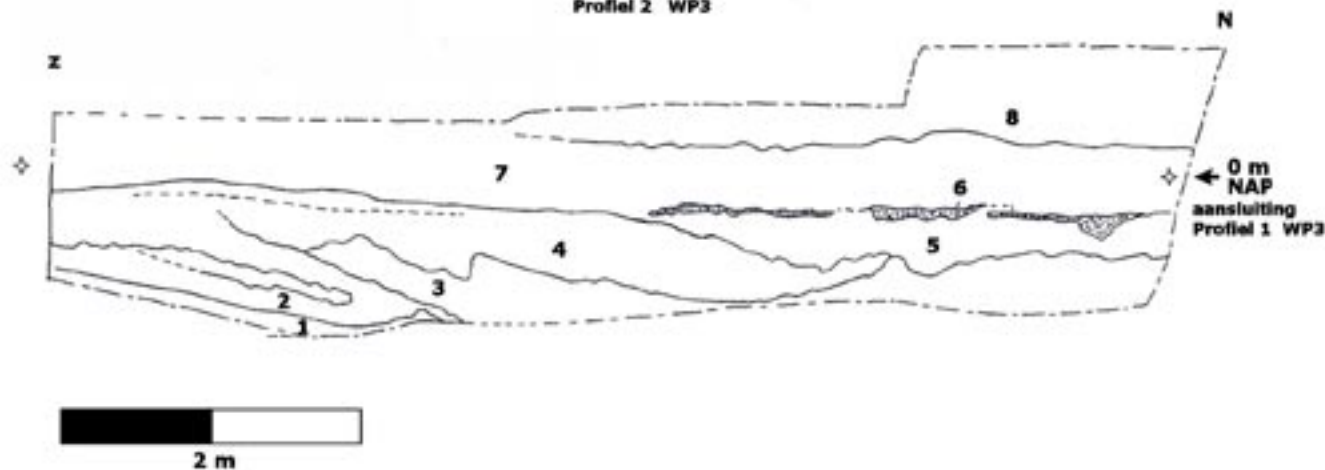
Profiel 2 WP3
